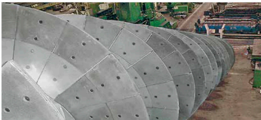
Conveyor screw being part of a slag granulating system; screw flights lined with KALMETALL C155; the screw has a diameter of 1,200 mm
