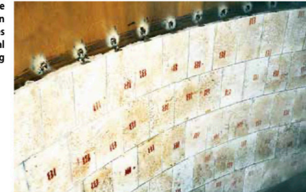
Short lining times for a whirler are achieved with a combined lining of hard compound KALCRET BTS and zirconium corundum KALCOR. The high application rate of KALCRET BTS is 5 m 2 /h
