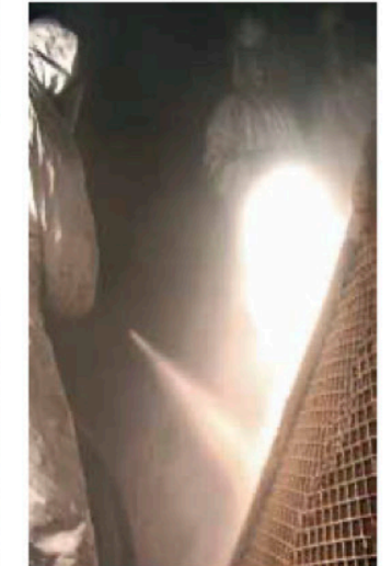
Short lining times for a whirler are achieved with a combined lining of hard compound KALCRET BTS and zirconium corundum KALCOR. The high application rate of KALCRET BTS is 5 m 2 /h
