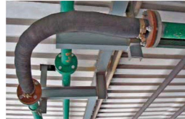
KALFLEX pipe bends in practical operation; here shown as flexible connection between rigid connection points
